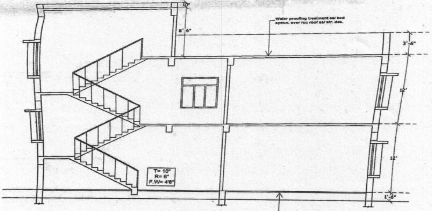
FLOORING AS/SPECIFICATION SECTION ON- A-A
